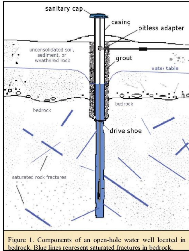
Example Well Diagram
