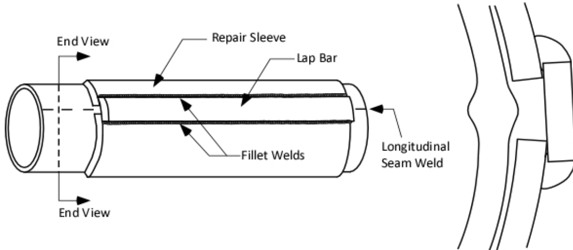
Figure 11. Seam weld reinforcement positioned in gap created by side strip.
